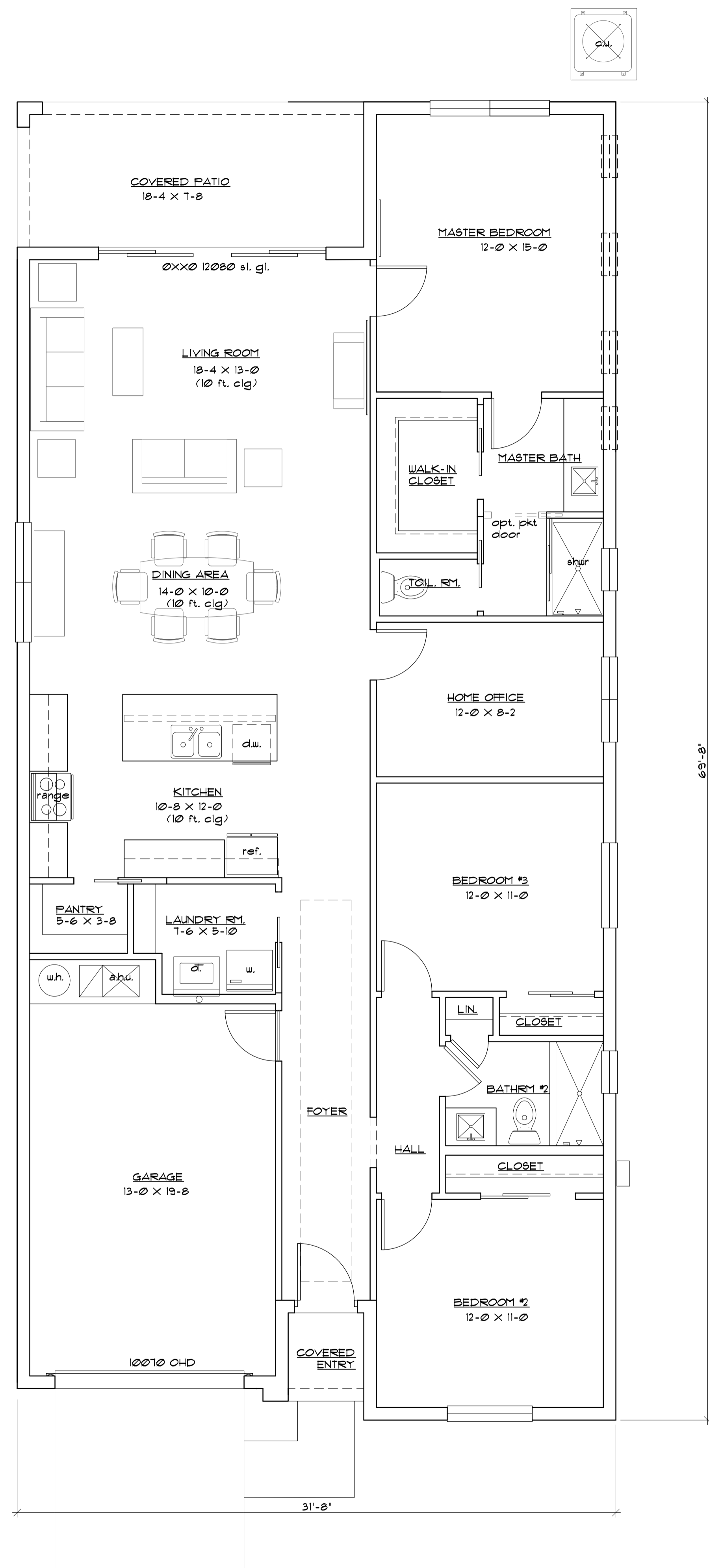
SINGLE UNIT FLOOR PLAN
